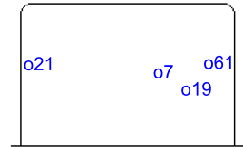
GK 35 of OLR
